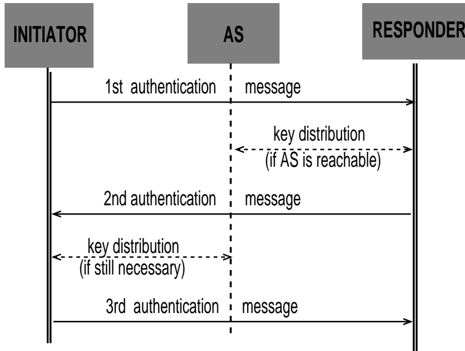
Fig. 5. Adaptive protocol
