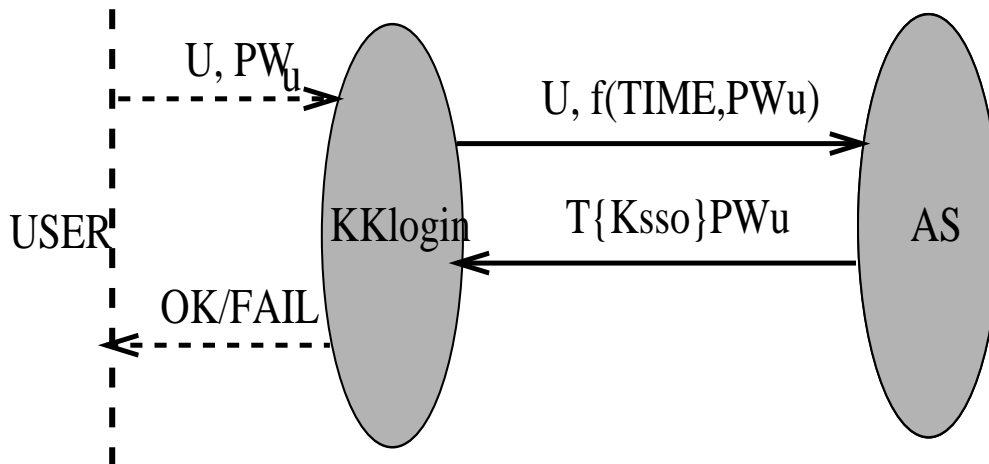
Fig. 1. Single Sign-On Protocol
