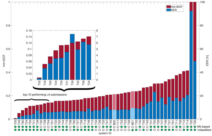
Fig. 4: Performance of the two baseline systems (B01 and B02) and the 48 primary systems for the LA scenario of the ASVspoof 2019 challenge. Results are in terms of the min-tDCF and EER (%).
