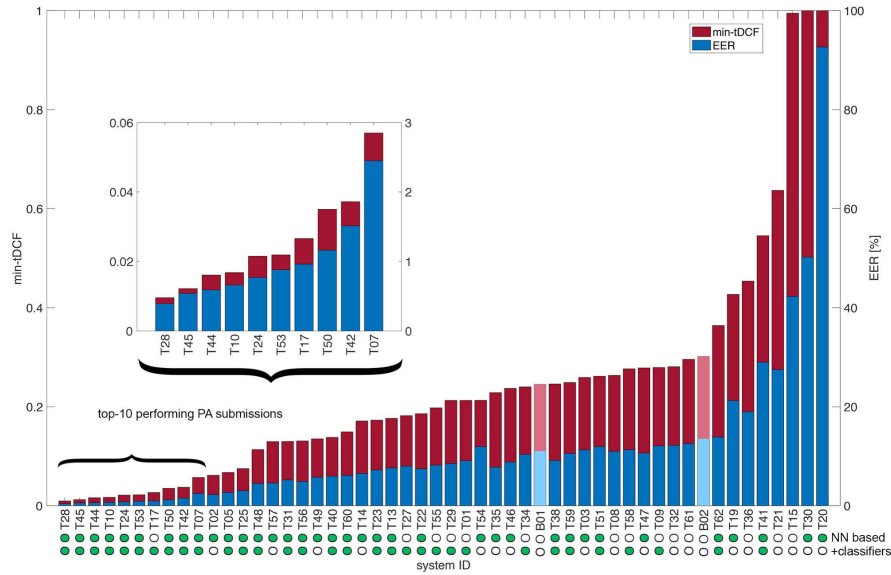
Fig. 5: Performance of the two baseline systems (B01 and B02) and the 50 primary systems for the PA scenario of the ASVspoof 2019 challenge. Results are in terms of the min-tDCF and EER (%).
