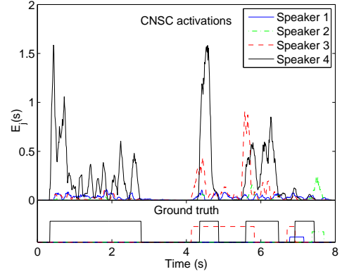
Fig. 1. An illustration of the correlation between ground-truth speaker activity (bottom) and CNSC activation energies (top) for 4 speakers in a conversation.
