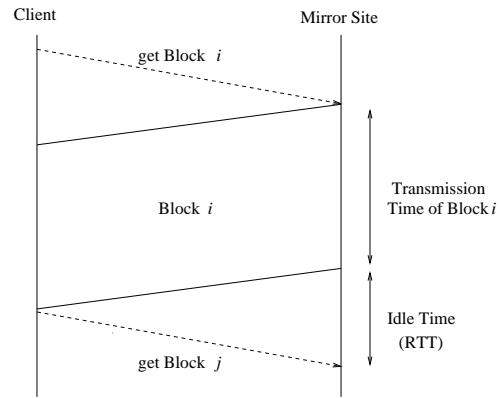
Fig. 3. Dynamic parallel-access : Block request.
