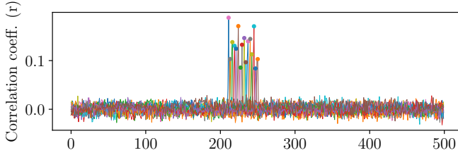
Figure 10. Correlation on amplitude for A_7 during a radio transmission with GFSK at f_{\text{carrier}} + 2 * f_{\text{clock}} Hz.
