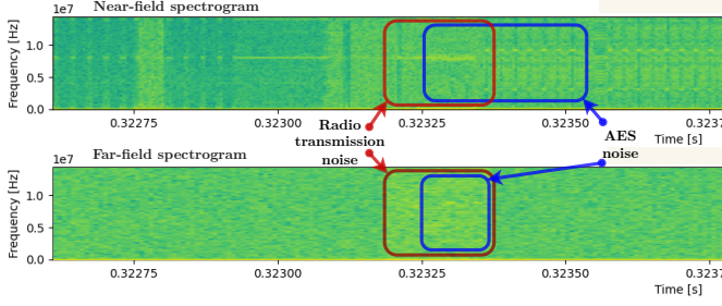
Figure 5. Leakage comparison between Conventional (upper) and Screaming Channel (bottom).
