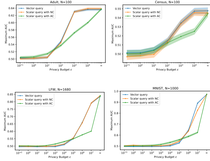
Figure 3: Comparison of the protection of the three approaches for Laplace when the adversary intercepts all components k = d for different values of \epsilon . The infinity \infty point presents the non-private case.
