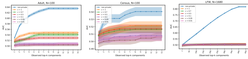
(a) The AUC of the attack when the AG algorithm is applied with respect to k
