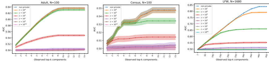
(b) AUC of the attack when the Laplace vector query algorithm is applied w.r.t. k .
