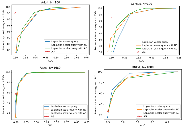
Figure 6: Trade-off posed by the four DP-PCA algorithms described Section. 5.2, between attack performance and data utility. We measure attack performance through AUC, and utility through the percentage of captured energy w.r.t. SVD.
