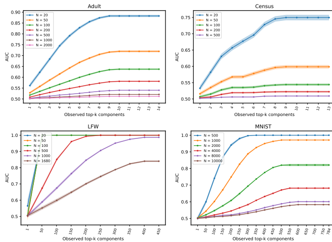
Figure 1: Impact of the sample size N and the observed top- k components on the attack’s performance. Shaded areas show 95% confidence intervals for the mean.
