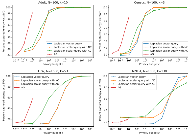
Figure 5: Trade-off posed by the four DP-PCA algorithms described in Section. 5.2, between the total privacy budget \epsilon and data utility. Utility is measured as the percentage of captured energy w.r.t. SVD.
