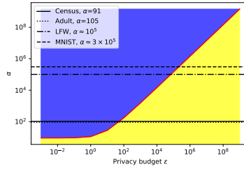
Figure 4: The yellow shaded area shows where naive composition introduces less noise than advanced composition.
