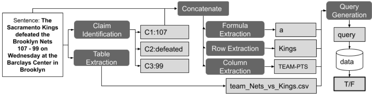
Figure 3: Architecture of the solution. Given a sentence, we identify the claims and the table to verify them. Then every claim (C1-C3 in the example) is processed individually to obtain a query for its verification. (We take claim C1 as an example in the figure.)
