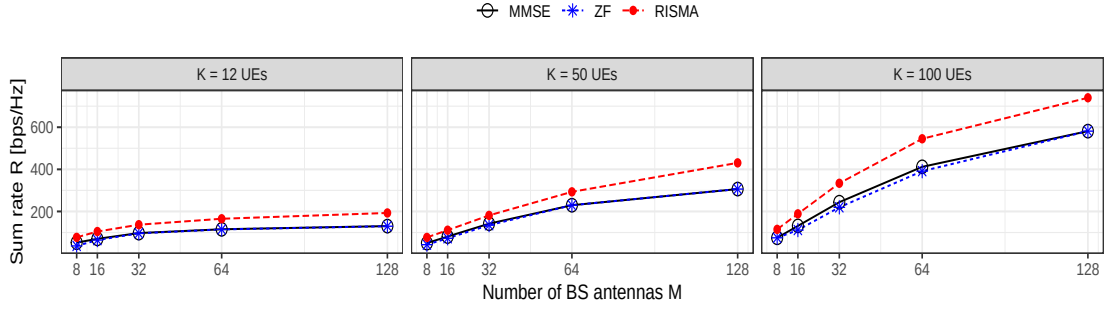
Figure 8.5 – Average sum rate in the multi-UE case obtained with the proposed RISMA algorithm (red line), with conventional MMSE precoding (black line) and with conventional ZF precoding (blue line) versus the number of BS antennas M , for fixed network area radius R_N = 150 m, transmit power P = 24 dBm and for different number of UEs K .
