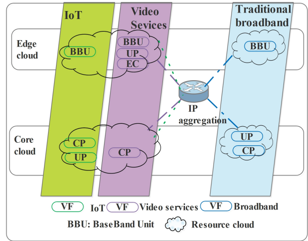
FIGURE 2: Indicative applications of 5G network slicing
