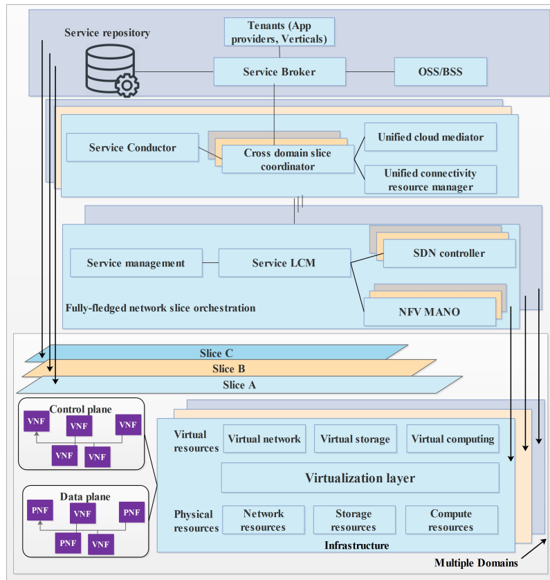
FIGURE 5: Orchestration architecture across multiple domain
