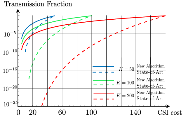
Fig. 1. The total CSI cost that is required to complete a fraction of the delivery phase inside a single coherence period. We compare the costs required by the proposed algorithm with the state-of-the-art algorithms [33], [34], where the later exhibit the same CSI requirements. The cost represents the number of users that need to send feedback. Parameter \gamma is fixed at value \gamma = \frac{1}{10} .
