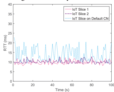
Fig. 9: Latency measurements of isolated IoT slices.
