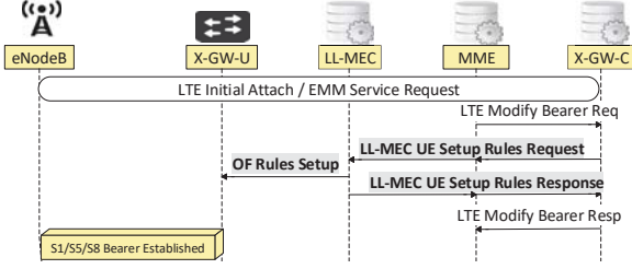
Fig. 2: Sequence diagram of S1/S5/S8 bearer setup.
