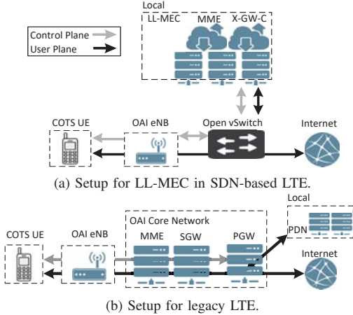
Fig. 3: The evaluation setup.
