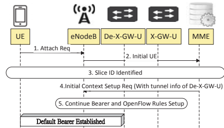
Fig. 8: Sequence diagram of DCN
