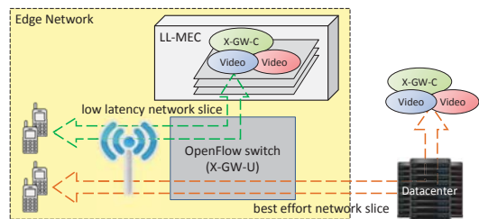
Fig. 6: Overview of end-to-end network slicing.
