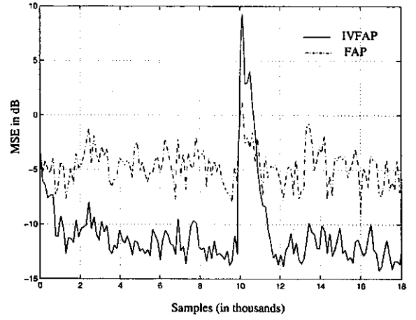
Figure 2: Comparison of the IVFAP and FAP algorithms.
