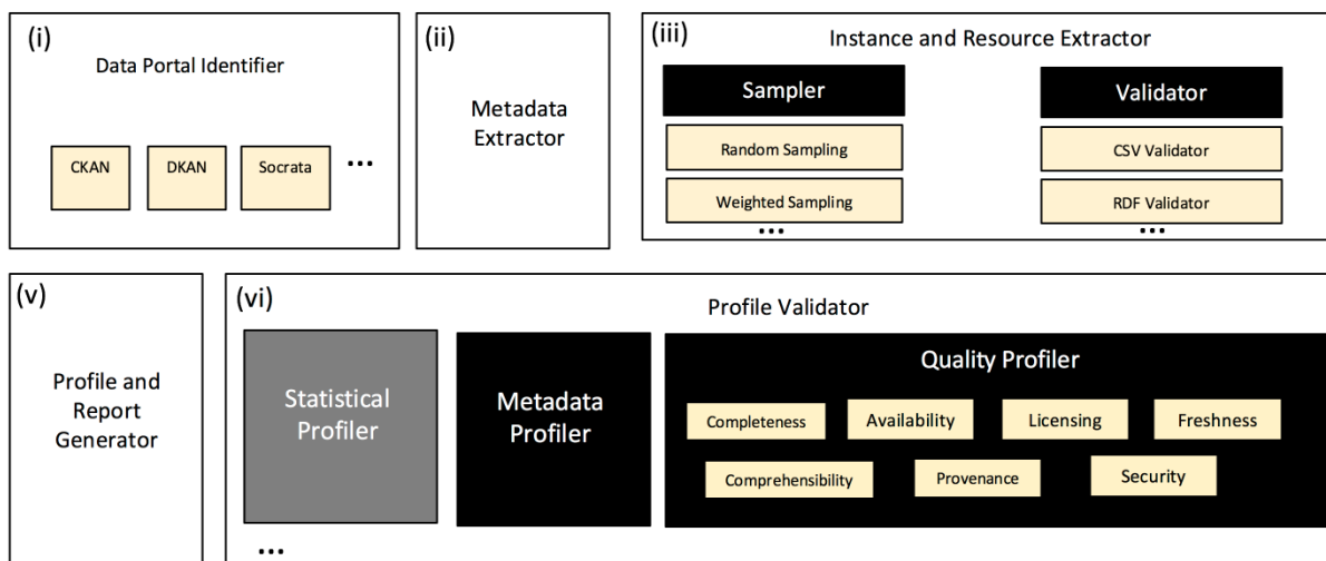
Fig. 1. Processing pipeline for objective dataset quality assessment
