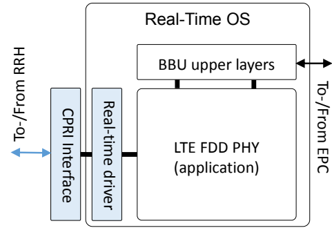
Fig. 2. RAN architecture on PC.
