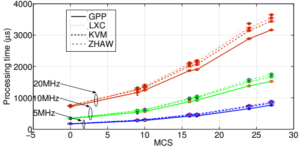
(b) Uplink
