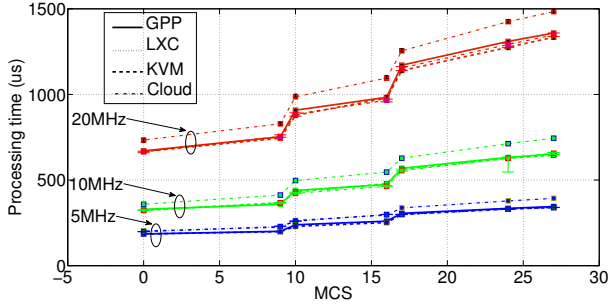
(a) Downlink
