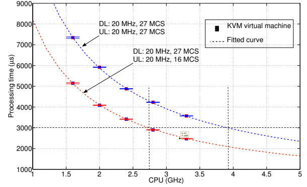
Fig. 6. Processing time for transmitting (OFDMA) and receiving (SC-FDMA) packets at eNB given full PRB allocation at 20 MHz.
