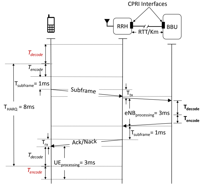
Fig. 1. HARQ process timing requirement.
