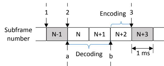
Fig. 3. Processing orders in OAI.
