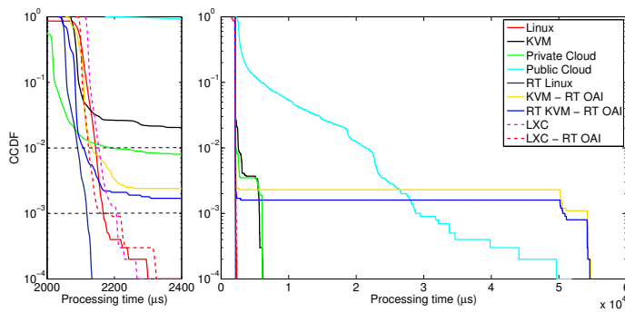
Fig. 7. Processing time distribution for received packets (at eNB) in the Cloud environment with BW=20 MHz, MCS=16.
