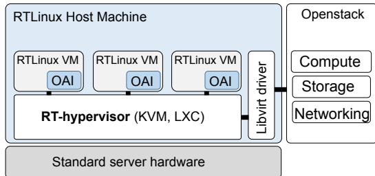
Fig. 4. OpenStack management architecture.
