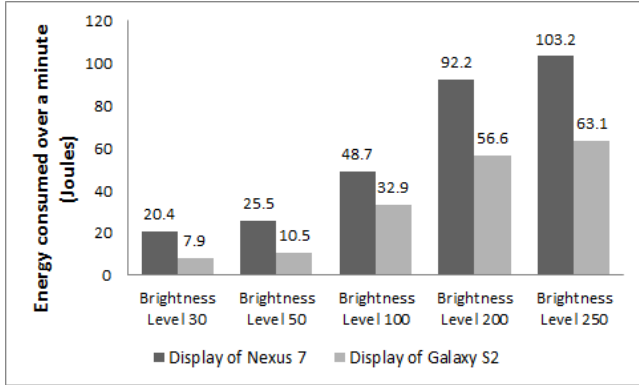
Figure 1. Energy consumption at display hardware.
