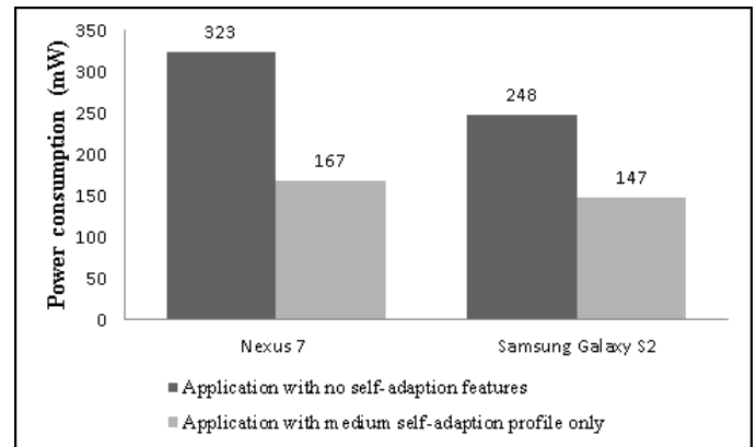
Figure 5. Comparison of power consumption between the application with no self-adaption and application with only medium self-adaption profile.
