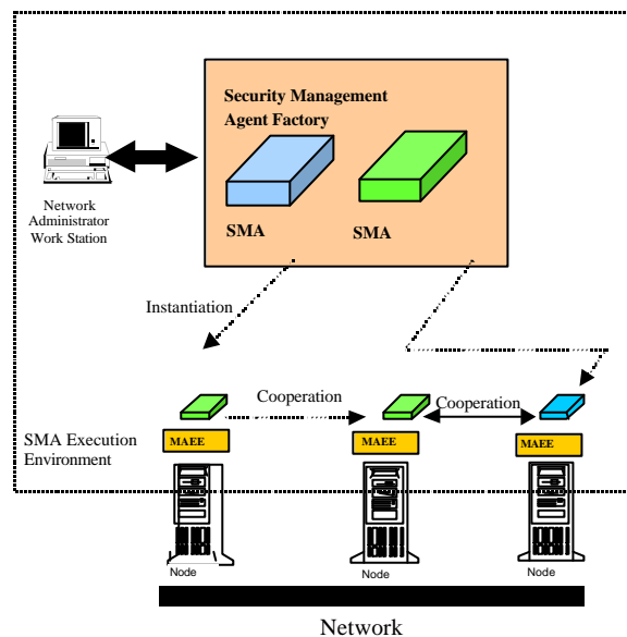
Figure 2: Intelligent Agent Security Management Architecture
