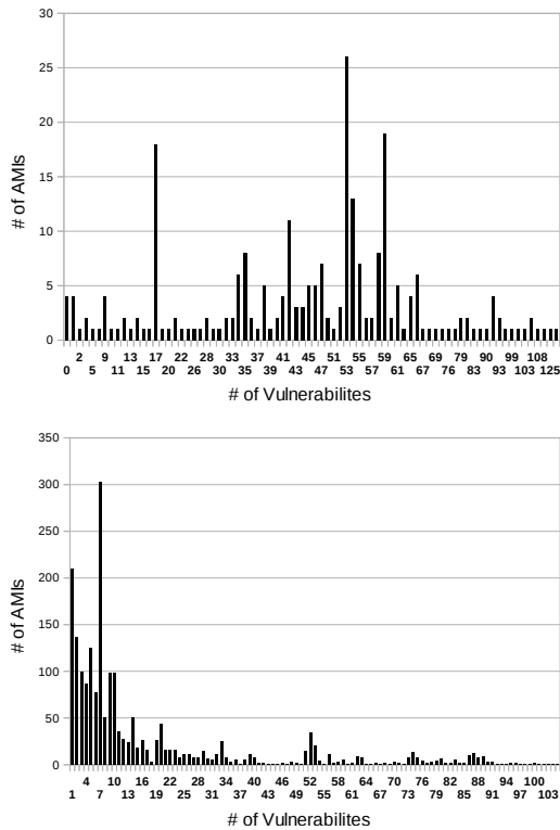
Figure 2: Distribution AMIs / Vulnerabilities (Windows and Linux)
