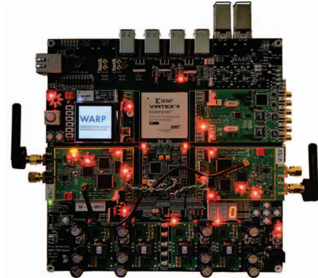
Fig. 2. WARP board with radio daughtercards.
