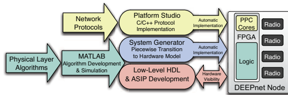
Fig. 3. WARP system tools and design flow.
