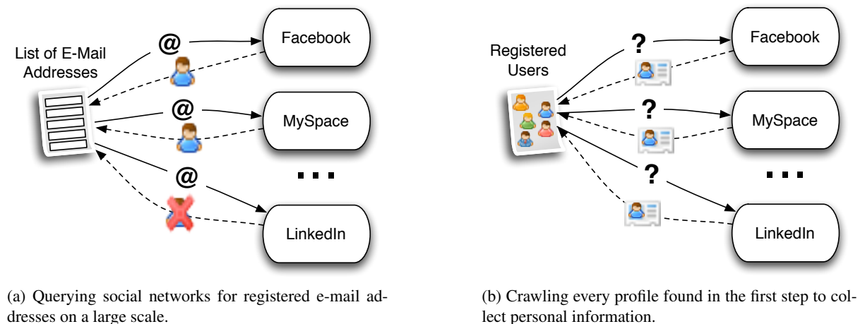
Figure 1: Automated user profiling based on information collected on social networks.
