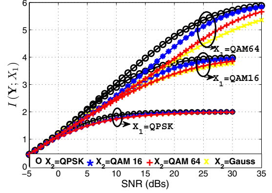
Fig. 4. Mutual information of the desired stream x_1 in the presence of interference stream x_2 for different constellations. SNR is defined as E\{\|\mathbf{h}_1 x_1\|^2\} / E\{\|\mathbf{z}\|^2\} . Interference strength is fixed as \sigma_2^2 = 0.5
