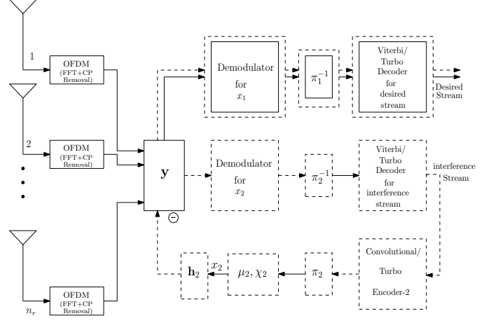
Fig. 3. Block diagram of receiver at MS. Continuous lines indicate PIC approach while dashed lines indicate AIC approach.
