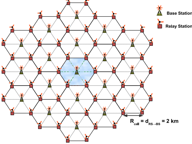
Fig. 1. RS deployment in B = 19 cells network. The BSs have N = 6 sectoral antennas each directed to a unique RS. Each RS consists of 3 RF elements each serving a unique cell.
