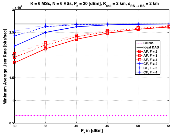
Fig. 3. Minimum average user rate versus P_r with SIC decoder after optimum decoding ordering.
