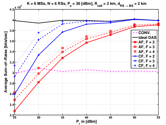
Fig. 2. Average sum-of-rates [bits/sec] versus P_r .
