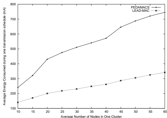
Figure 5: Average energy consumption in a cluster as a function of the number of nodes
