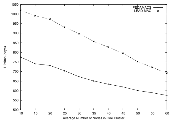
Figure 3: Average lifetime of a cluster as a function of increasing the number of nodes
