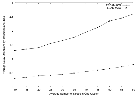
Figure 4: Average delay in a cluster as a function of the number of nodes
