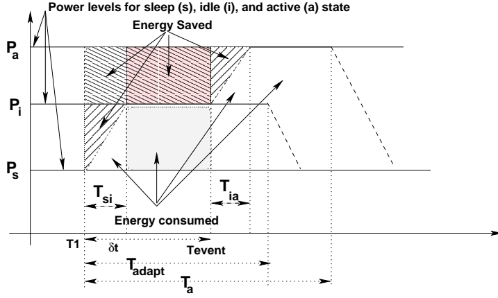
Figure 2: Energy Savings through adaptive duty cycle
