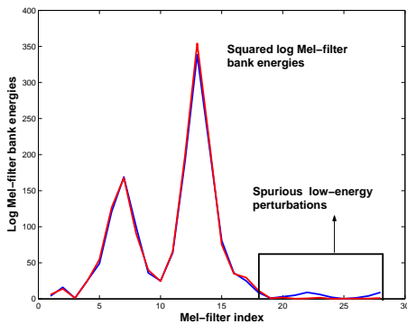
Fig. 2. Square of the log Mel-filter bank energies of clean and noisy (perturbed) speech.
