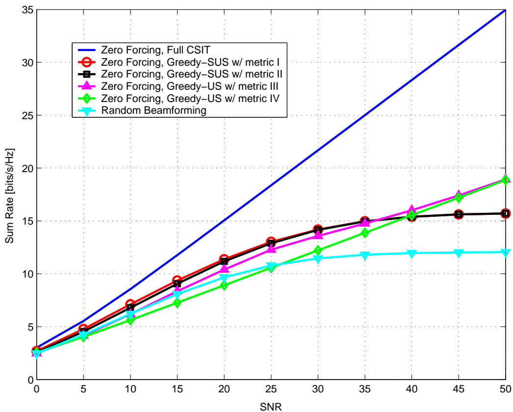
Fig. 1. Sum rate versus the average SNR for B = 4 bits, M = 2 transmit antennas and K = 30 users. Metric III combined with Greedy-US exhibits a linear sum-rate growth in the interference-limited region in contrast to Metric I and II, whose sum rate saturates at high SNR.
