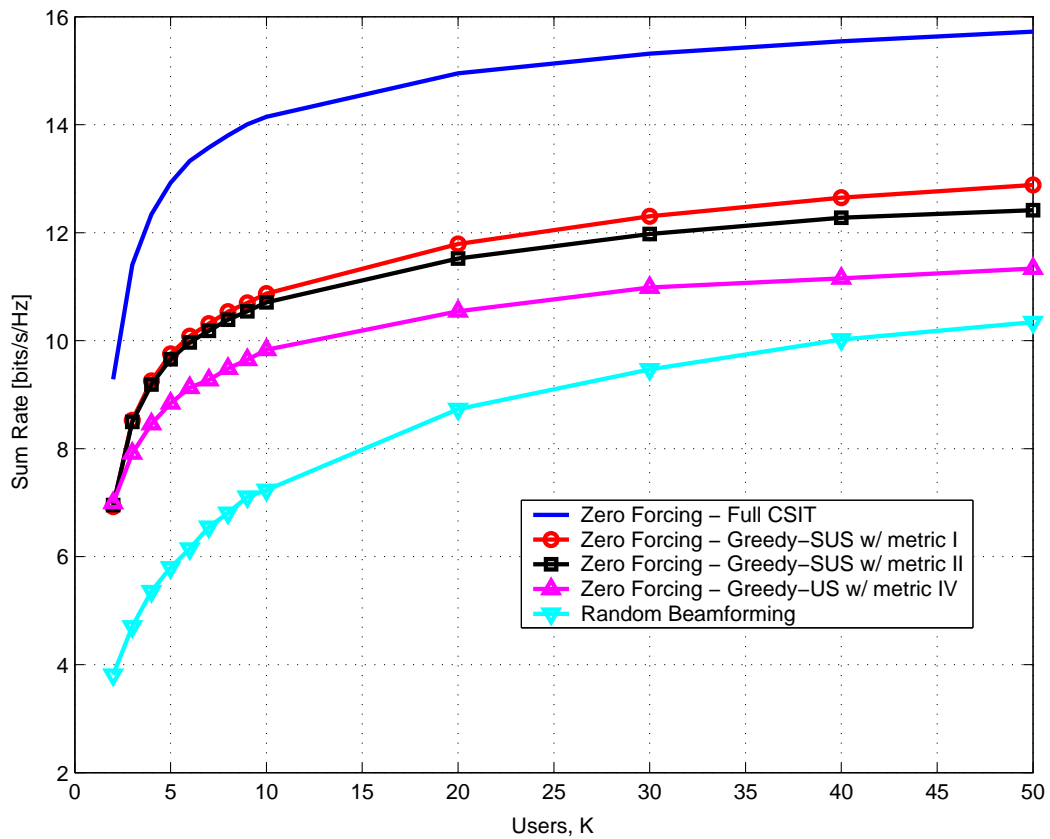
Fig. 3. Sum rate versus the number of users for different approaches with SNR = 20 dB, M = 2 transmit antennas and limited 10-bit total feedback bits where B = 5 bits are used for codebook indexing and (10 - B) bits for CQI quantization. For metric IV, 2 bits are used for quantization of the channel norm and 3 bits for the alignment.
