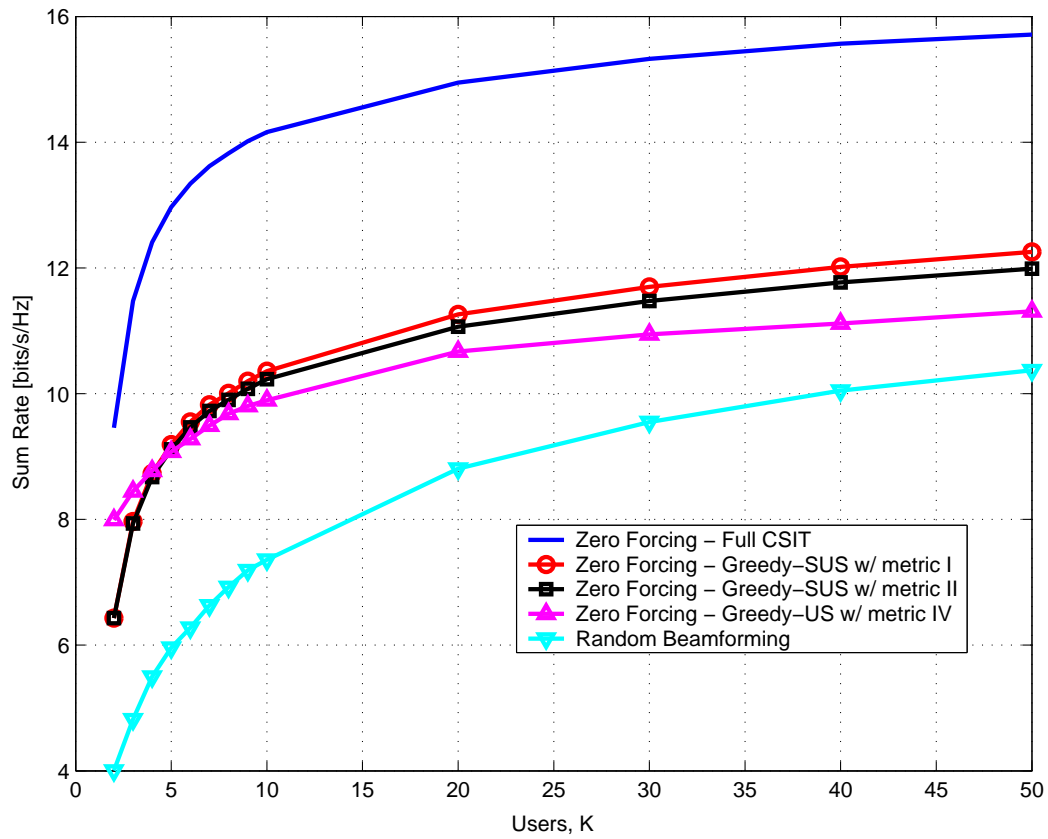
Fig. 2. Sum rate as a function of the number of users for B = 4 bits, M = 2 transmit antennas and SNR = 20 dB. All CQI scalar metrics can exploit the multiuser diversity gain, achieving optimal capacity growth.
