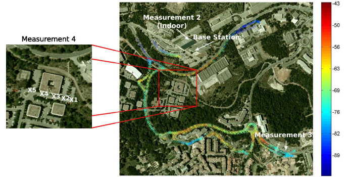
Fig. 2. Map of the measurement scenario. In measurement 1 the users were driving in cars along the indicated routes (the colors show the received signal strength in dBm along the routes). Measurements 2–4 are indicated on the map.
