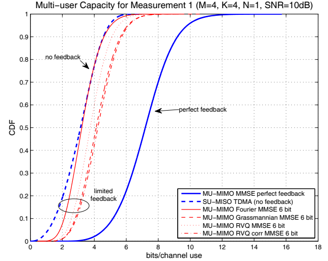
Fig. 6. CDF of the sum rate of MU-MIMO with MMSE precoding with different feedback schemes for measurement 1. The average SNR is fixed to 10dB for each user. We compare the performance under several codebooks of size 64 (6 bit) with the perfect feedback case as well as to the case with no feedback, which is equivalent to SU-MISO TDMA.
