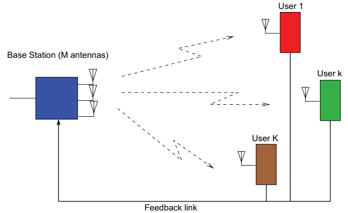
Fig. 1. Multi-user MIMO system model.
