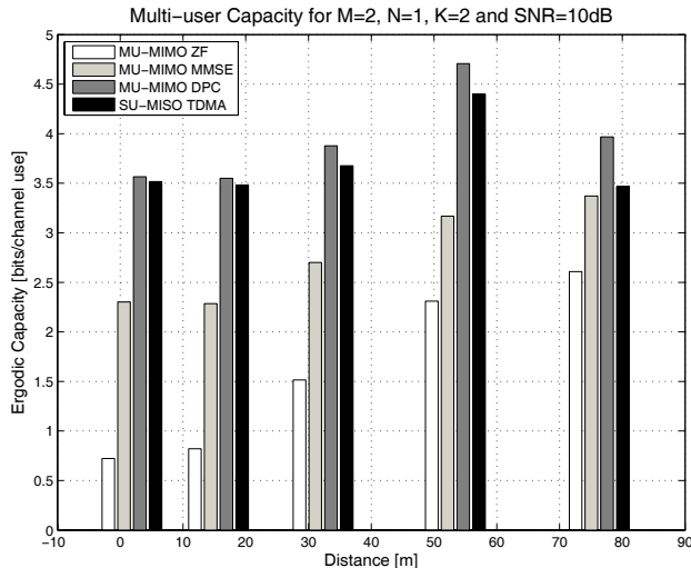
Fig. 5. Comparison of mean MU-MIMO sum rate for DPC and SU-MISO TDMA, as well as ZF and MMSE precoding with respect to inter-user distance for measurement 4. The average SNR is fixed to 10dB for each user.
