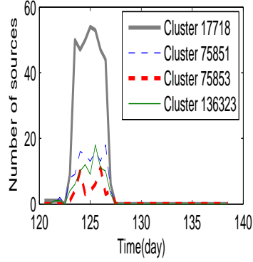
Fig. 14. Example Fingerprint worm
