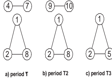
Fig. 7. Correlated groups extraction
