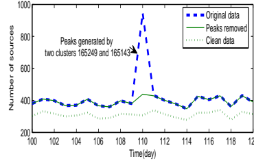
Fig. 4. Data Pre-processing
