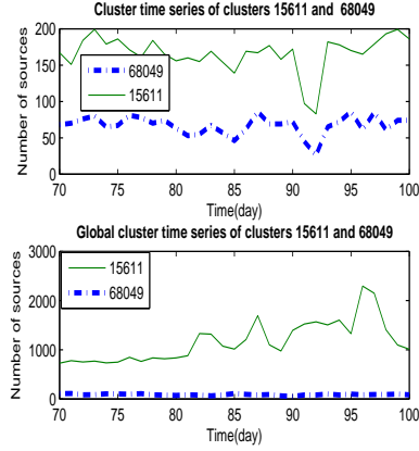
Fig. 2. Global cluster time series vs. cluster time series
