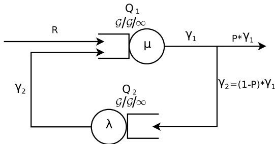
Figure 3: Queuing system representing the overall system behavior.
