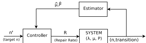
Figure 1: The adaptive control scheme.
