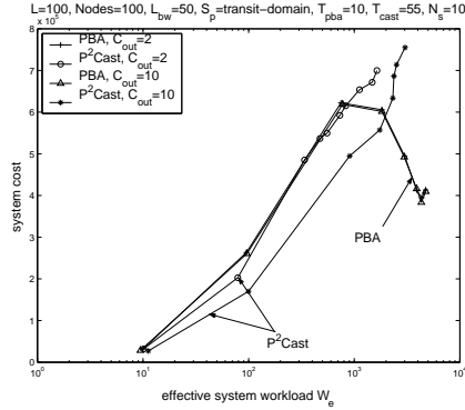
Fig. 3. The system cost for PBA and P^2cast , for a network of 100 nodes, L_{bw} = 50 , the server is placed in the transit-domain, the number of servants is N_s = 10 , T_{pba} = 10 min, and T_{cast} = 55 min.
