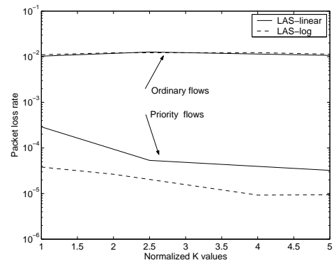
Figure 14: Packet loss rate as a function of normalized k values for LAS-linear and LAS-log policies; load \rho = 0.73 , q = 0.1 .
