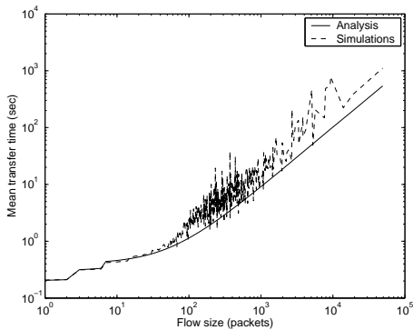
Figure 5: Mean transfer time validation for load \rho = 0.73 and loss rate = 3.6%
