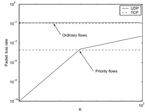
Figure 15: LAS-fixed( k ): Packet loss rate as a function of normalized k values for UDP and TCP flows; load \rho = 0.73 , q = 0.1 .
