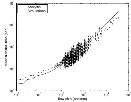
Figure 3: Validation of FCFS model, load \rho = 0.73 , loss rate = 1.2%
