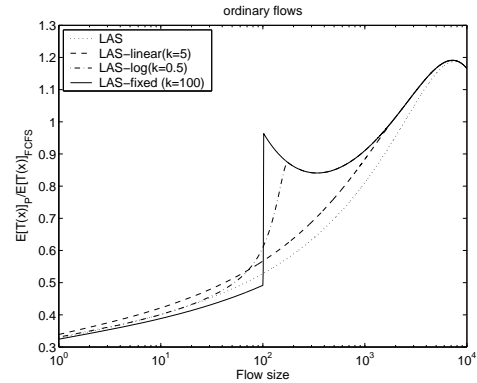
(b) Ordinary flows
