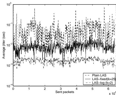
Figure 16: Average jitter of UDP flow for non-overlapping windows of 100 sent packets, load \rho = 0.7
