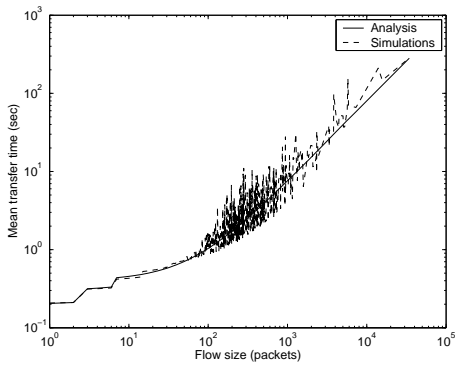
Figure 4: Validation of LAS model, load \rho = 0.73 , loss = 1.2%
