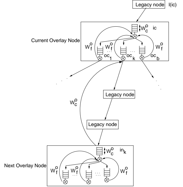
Figure 2: Overlay MCC model
