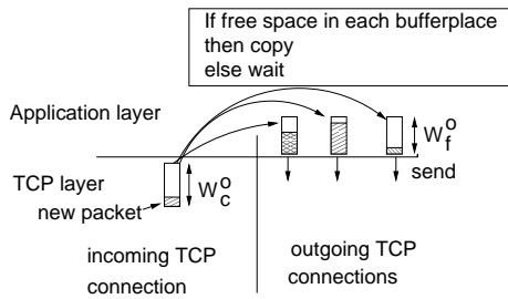
Figure 4: Implementation of the Overlay MCC model
