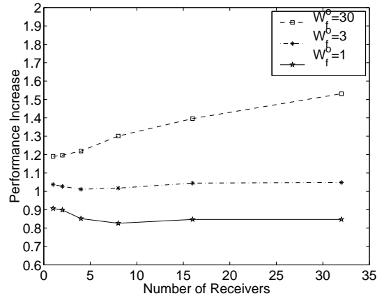
Figure 7: Performance comparison for heavy tailed service times ( P = 5 , W_c^o = 3 ).
