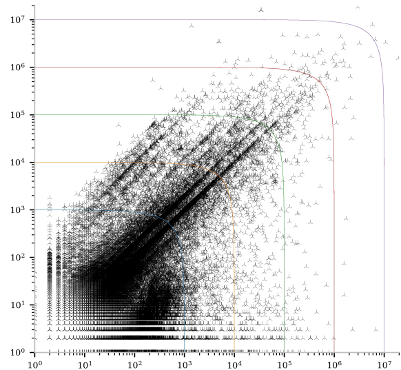
Figure 11: Interactions of active contracts. The horizontal axis indicates the number of incoming calls, the vertical axis the number of outgoing calls, both in a logarithmic scale. The colored lines connect points with the same sum of incoming and outgoing calls.
