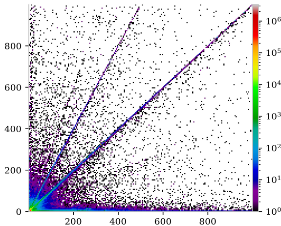
Figure 12: Heatmap of contracts with at most 1000 incoming and outgoing calls each. The colormap uses a logarithmic scale.
