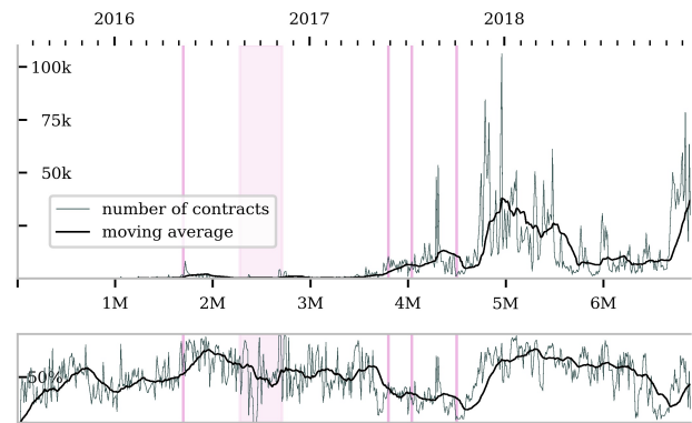
Figure 3: Occurrence of loners. The upper plot shows the number of loners created within a block range, the lower plot their percentage with regard to all creations.
