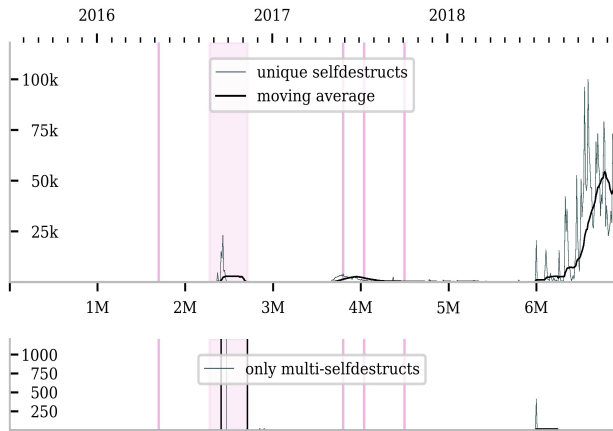
Figure 4: Contract destruction. The upper plot shows the number of contracts that selfdestructed within a block range. The lower plot depicts the accumulated selfdestructs of contracts that selfdestructed multiple times. The vertical axis of the lower plot was clipped, since numbers greater than 1000 only appeared during the DoS period of 2016.
