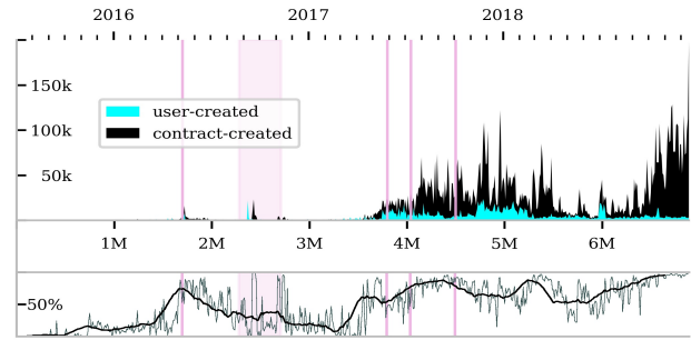
Figure 2: Distribution of contract creations. The upper part shows a stackplot of user-created contracts in blue and contract-created contracts in black. The lower part indicates the percentage of contract-created contracts with regard to all contract creations, per 10 k block range.
