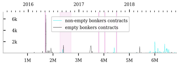
Figure 9: Occurrence of bonkers contracts. The black line depicts the number of empty bonkers contracts created within a block range, the cyan line the number of non-empty bonkers contracts.
