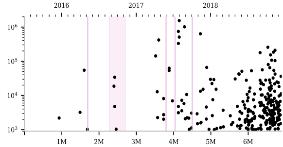
Figure 10: Creation of breeders. The vertical axis uses a logarithmic scale for the number of contracts that a breeder created so far.
