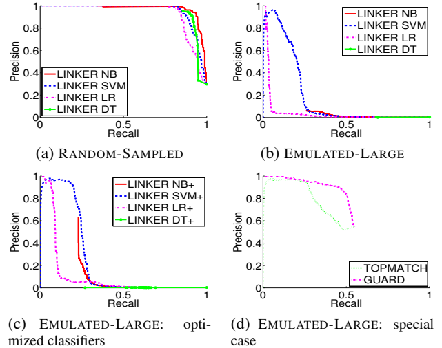
Figure 2: Precision and recall tradeoff for matching Twitter to Facebook profiles using different classifiers when evaluated over RANDOM-SAMPLED and EMULATED-LARGE.
