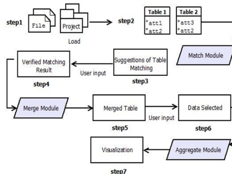
Figure 2: Framework Architecture
