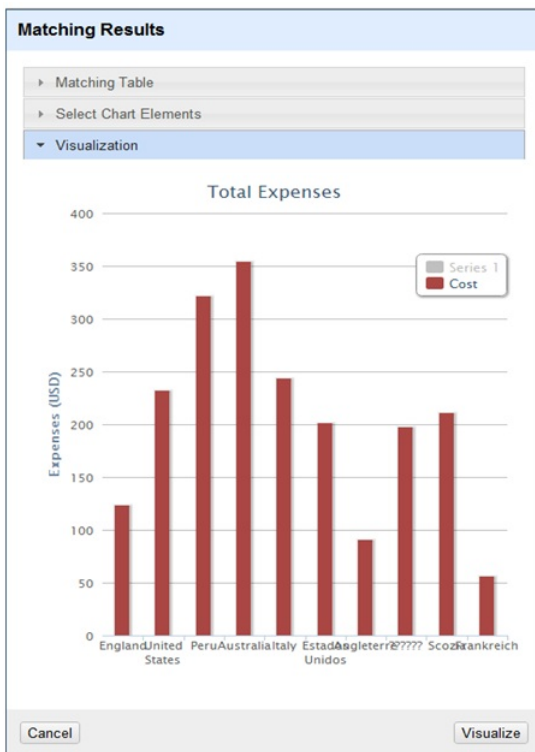
Figure 5: Data Selection
