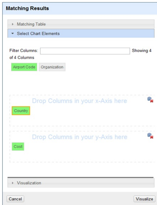
Figure 4: Data Selection
