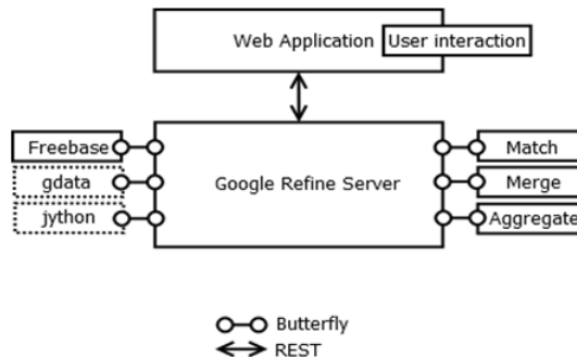
Figure 1: Framework Architecture
