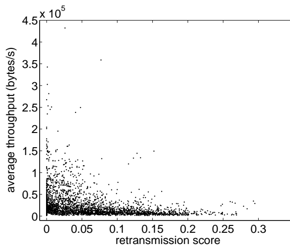
Figure 15: Retransmission score vs. throughput
