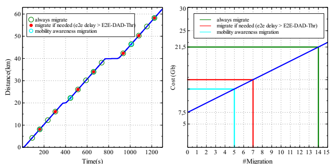
Fig. 9. The distance traveled by the VUE over time and migrations epochs of the number of edge-Cloud service migrations for each approach.
