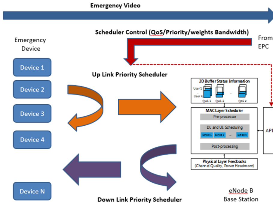
Figure 2: Scheduler Overview
