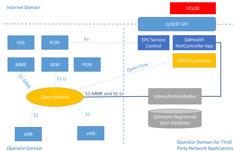
Figure 3: EPC Architecture Overview
