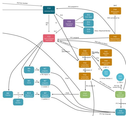
Fig. 1. Modeling a musical work: M-classes and U-properties are extensions of FRBRoo
