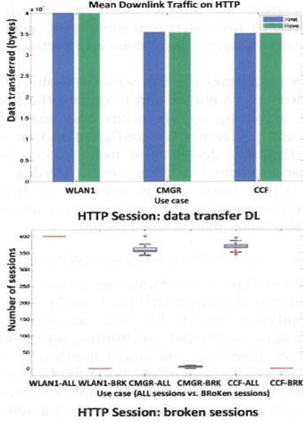
Figure 4. Simulation results for web browsing
