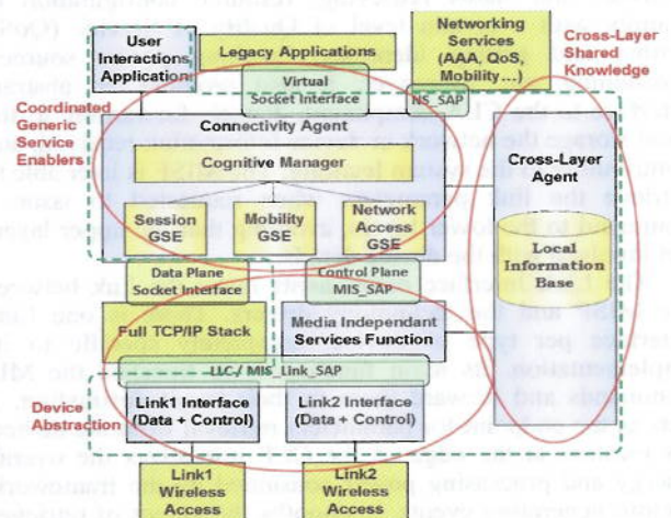
Figure 2. Global architecture of the CCF
