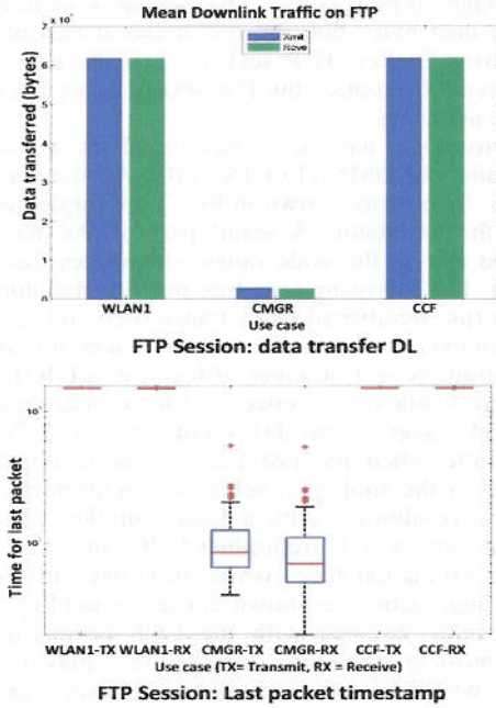
Figure 5. Simulation results for file transfer
