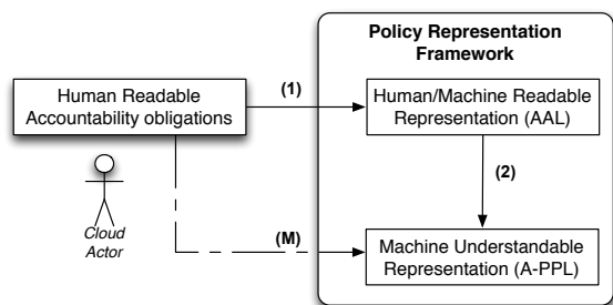
Figure 1: Overview on the accountability policy representation framework.
