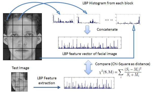
Figure 2: LBP face recognition
