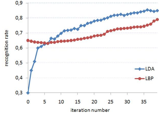
Figure 4: Average accuracy on test set as function of iteration number of co-training, initialized with 2 labelled examples per subject
