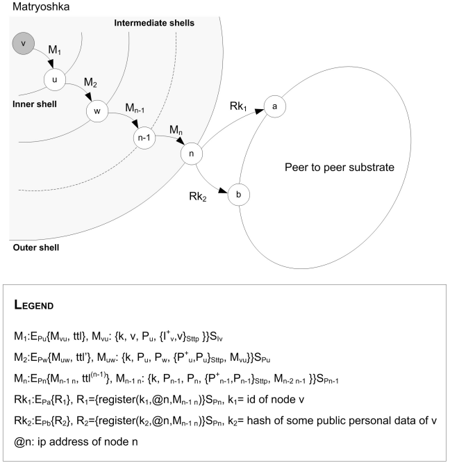
Fig. 2. Account and matryoshka creation with key registration for node \mathcal{V}
