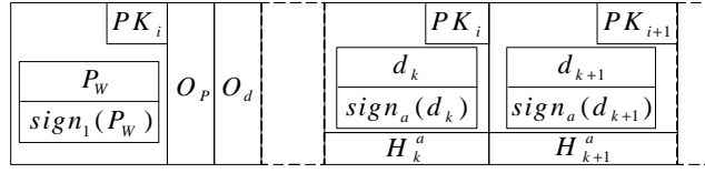
Fig. 5. Workflow message structure
