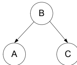
Figure 4. The Bayesian network (BN) spells out the factorization that is a simplification of the chain rule of probability.
