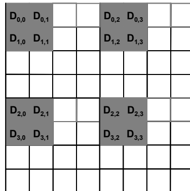
Figure 61. DCT coefficients of an 8 x 8 image block.
