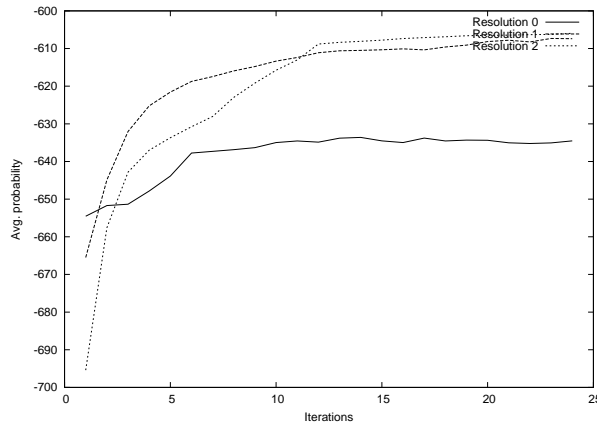
Figure 50. Total likelihood during training.
