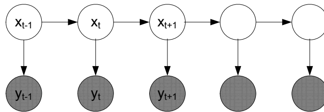
Figure 5. The one-dimensional hidden Markov model.
