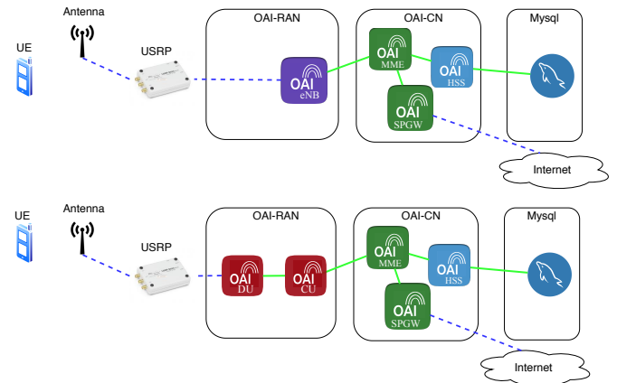
Fig. 2. 4G/5G network illustration: Monolithic RAN (top), versus disaggregated RAN (bottom) where three principal features are demonstrated: i) change of network configuration, ii) network upgrade (i.e., upgrade one or more network entities), iii) switch between monolithic RAN (top topology in Fig. 1) and disaggregated RAN (bottom topology in Fig. 1) and vice versa according to user traffic.
