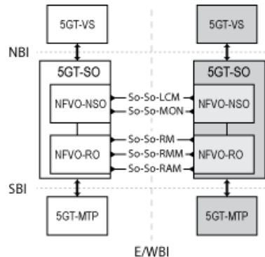
Figure 2: 5GT-SO functional architecture
