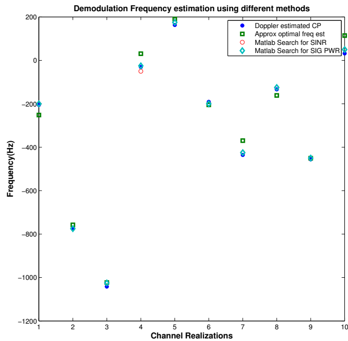
Fig. 2. Comparison of methods to estimate demodulation frequency
