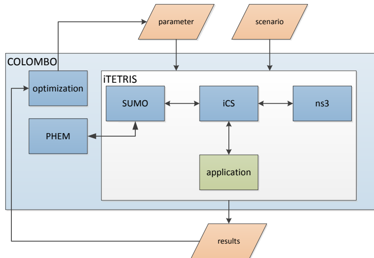
Figure 6 - The simulation architecture used and extended in COLOMBO
