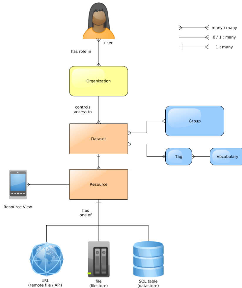
Figure 3.2: CKAN data model
