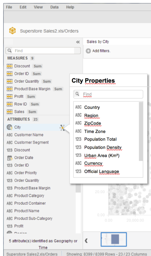
Figure 9.2: UI Prototype of semantic data enrichment in SAP Lumira
