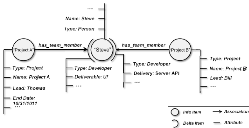
Figure 6.3: AIS data model
