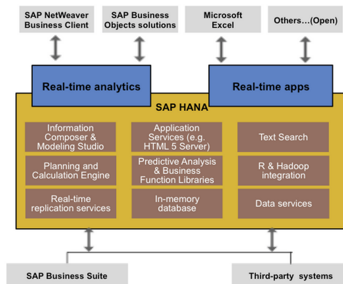
Figure 6.2: SAP's High Performance Analytic Appliance (HANA) with the SAP BI suite
