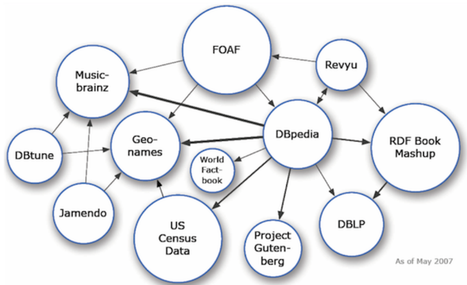
Figure 2.2: The LOD cloud as of May, 2007
