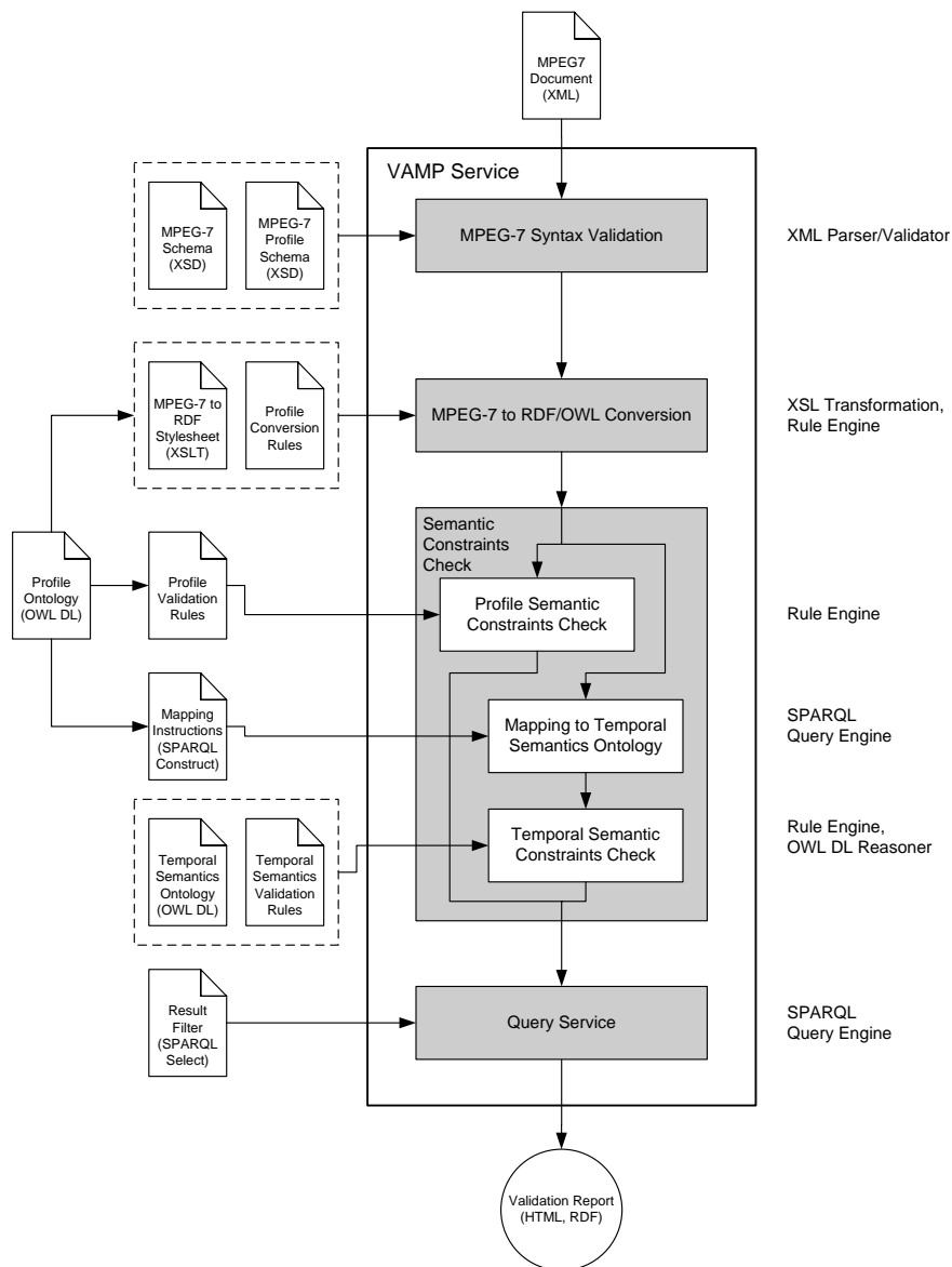
Fig. 1 General architecture of the VAMP service
