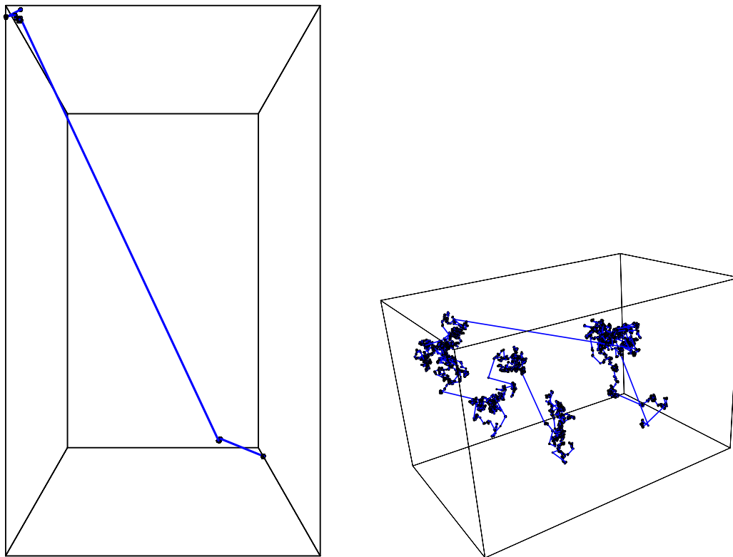
(a) With \beta = 0.55 one big step dominates the distribution.
